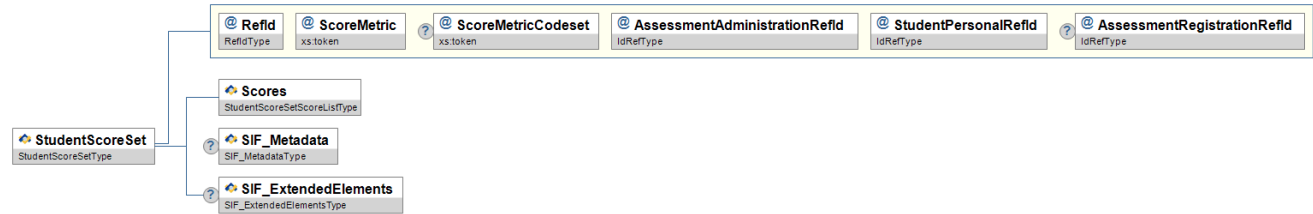
Figure 3.2.10.1: StudentScoreSet
