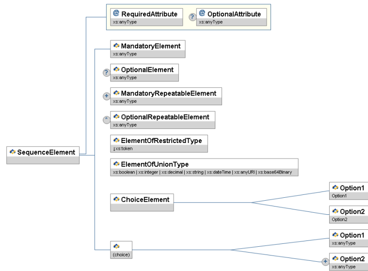
Figure 2.2.6-1: XML Diagram Conventions
