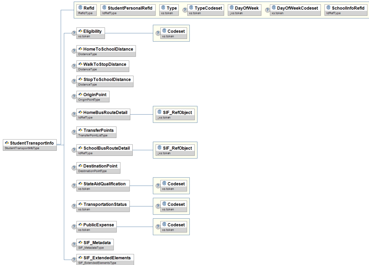
Figure 3.17.7-1: StudentTransportInfo
