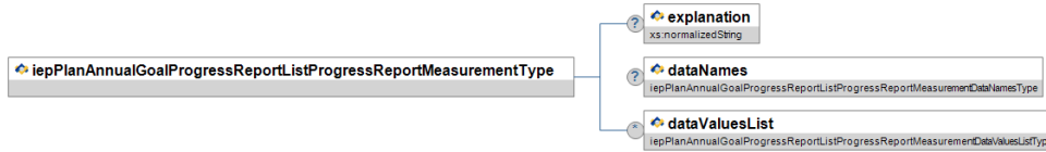
Figure A.292-1: iepPlanAnnualGoalProgressReportListProgressReportMeasurementType
