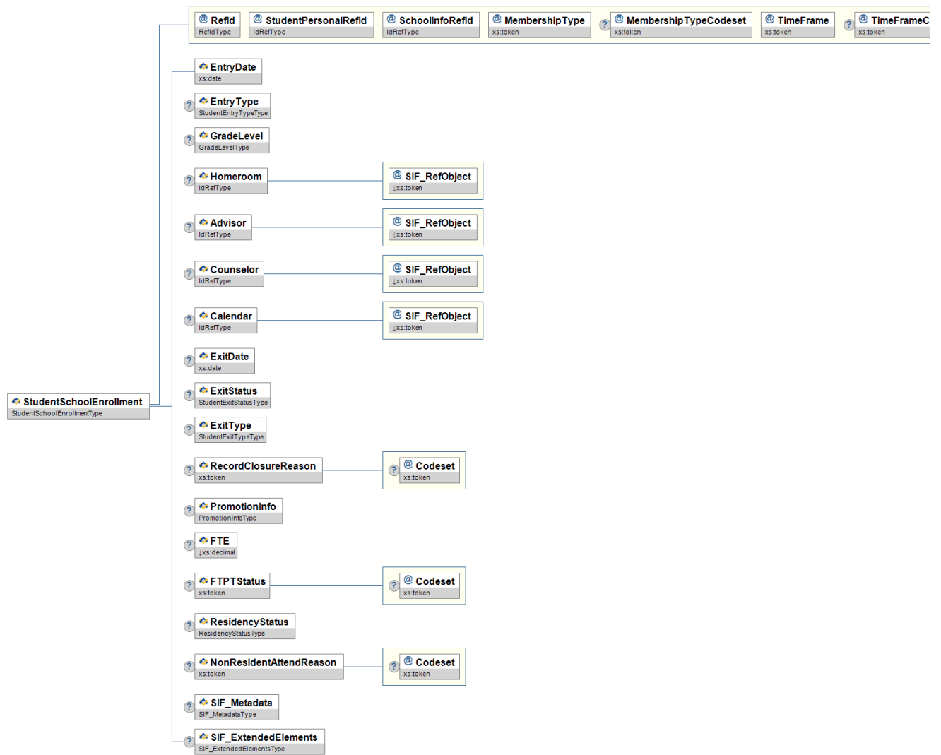
Figure 3.15.28-1: StudentSchoolEnrollment
