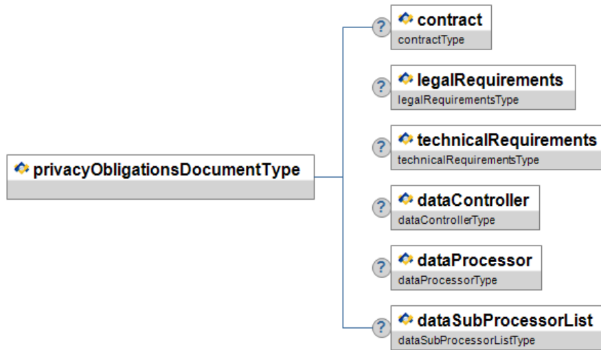
Figure A.83-1: privacyObligationsDocumentType
