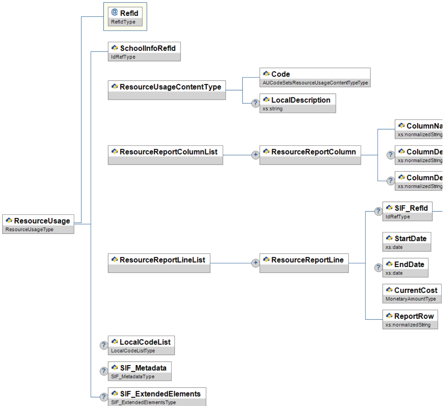
Figure 3.13.1-1: ResourceUsage
