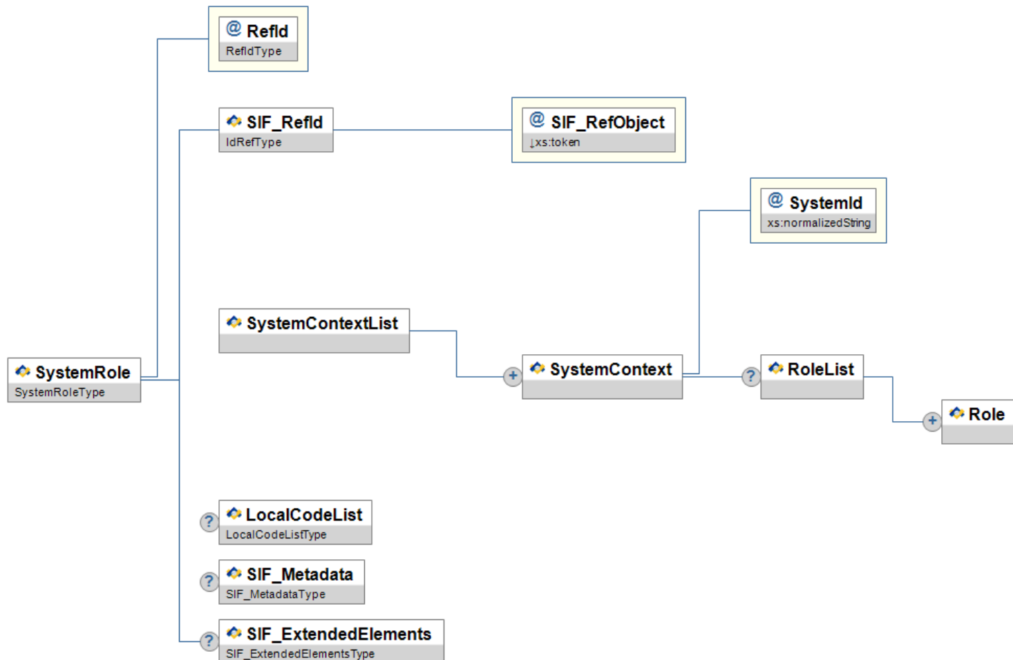
Figure 3.13.2-1: SystemRole
