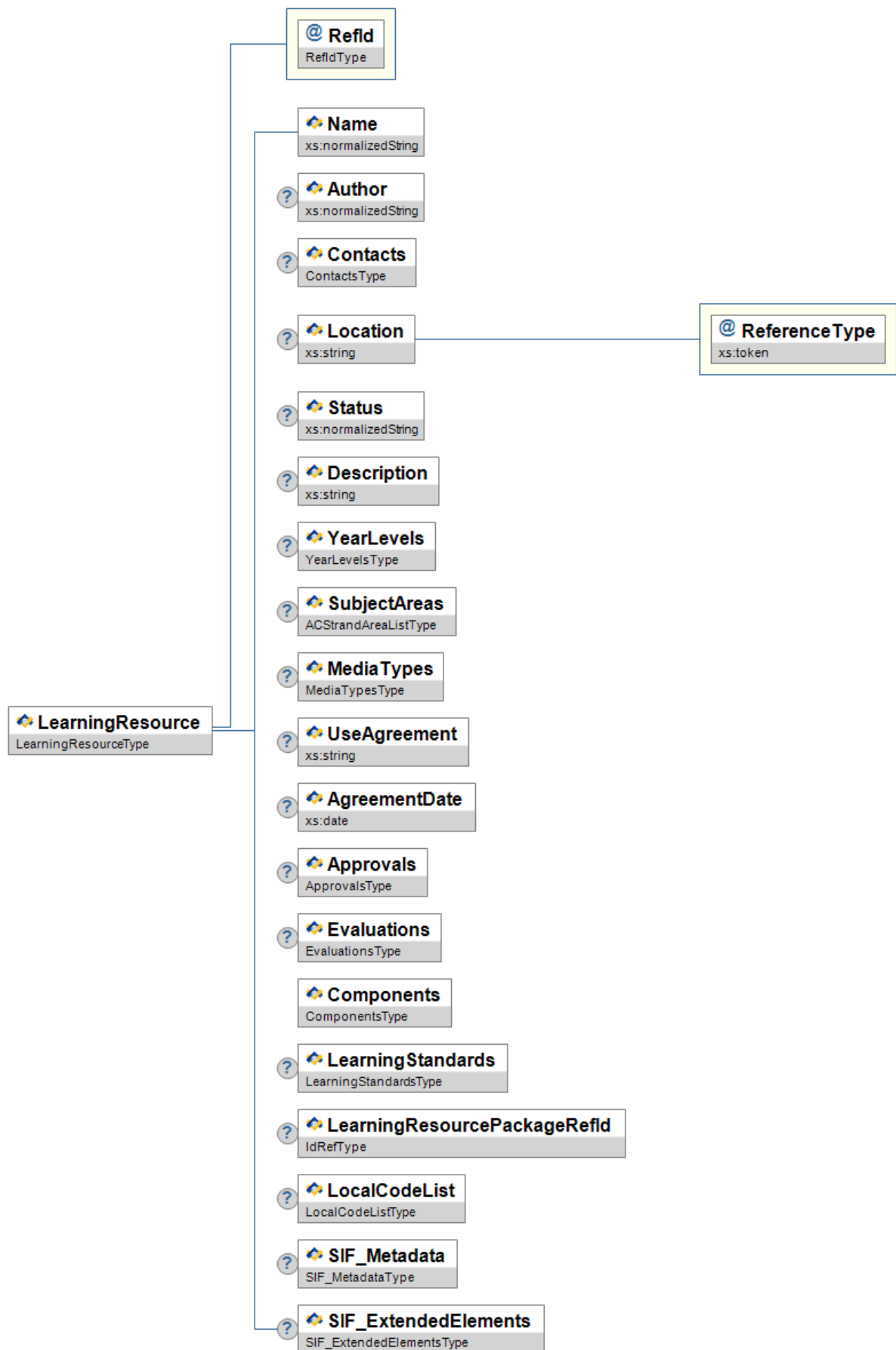
Figure 3.8.1-1: LearningResource
