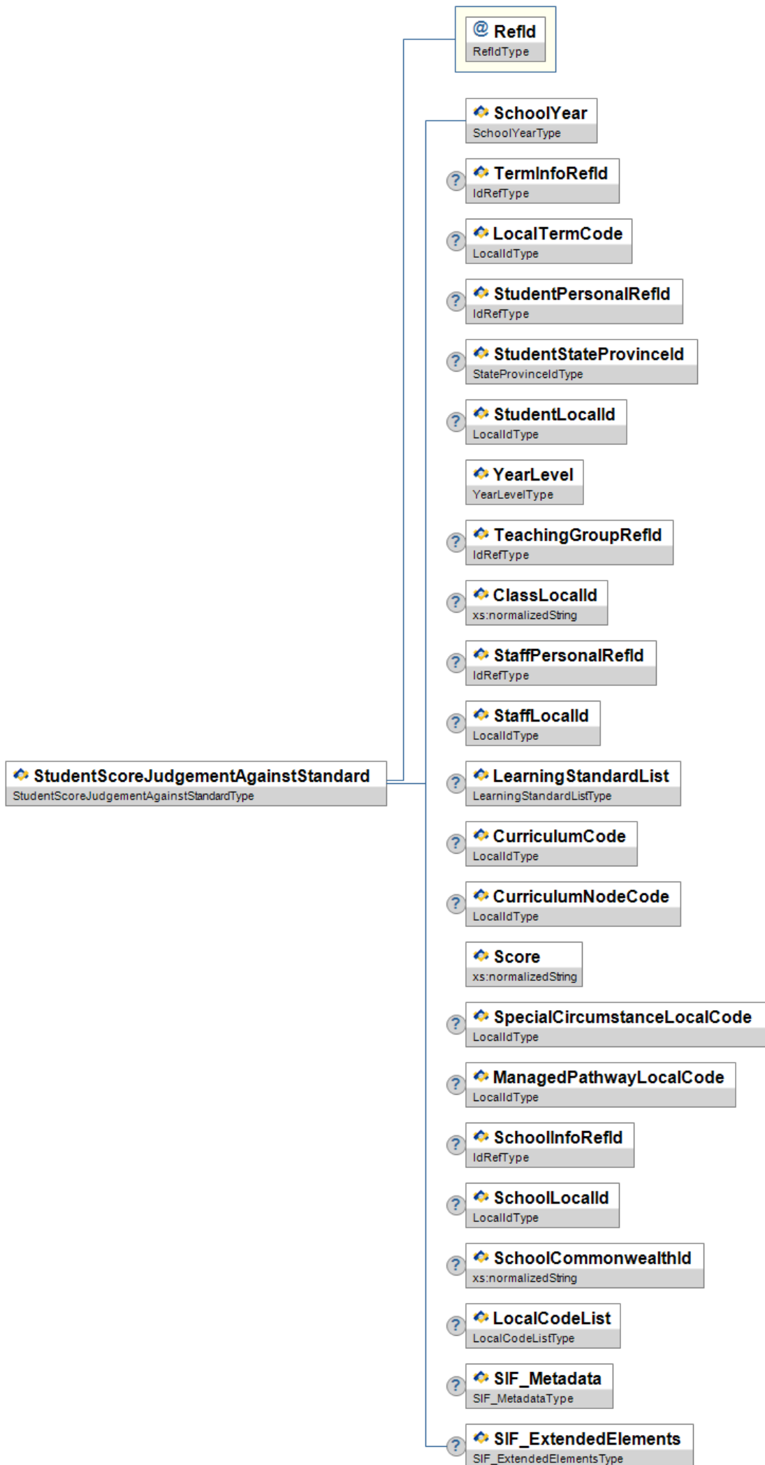
Figure 3.6.5-1: StudentScoreJudgementAgainstStandard
