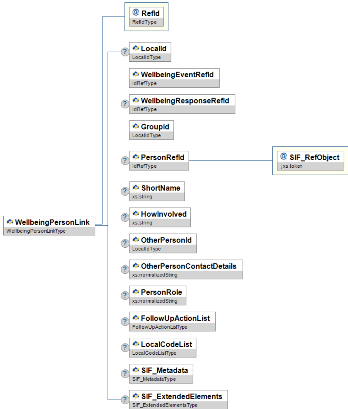
Figure 3.12.6-1: WellbeingPersonLink
