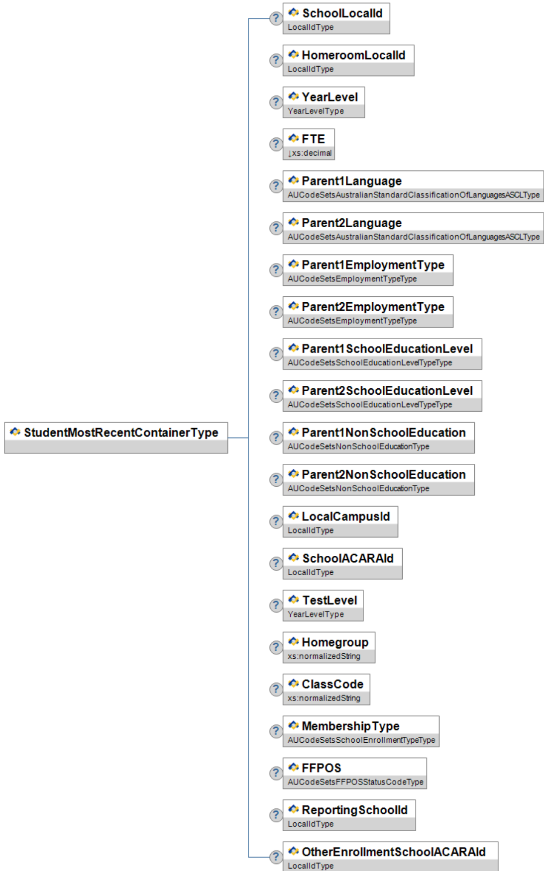
Figure A.239-1: StudentMostRecentContainerType
