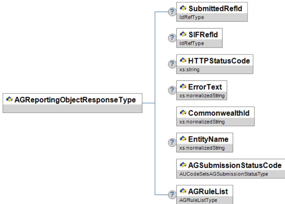
Figure A.12-1: AGReportingObjectResponseType
