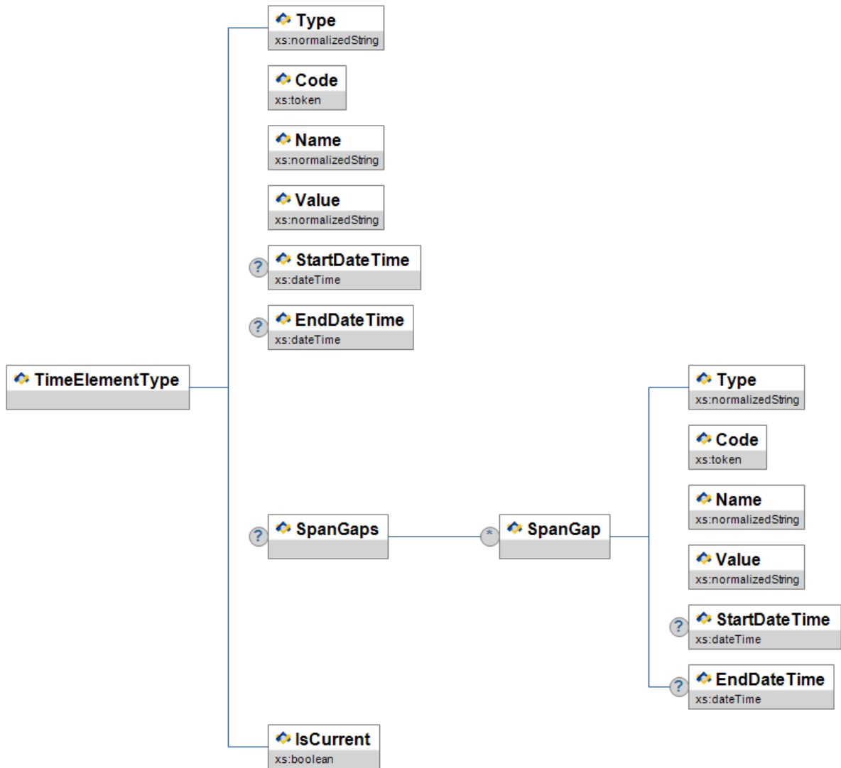
Figure A.258-1: TimeElementType
