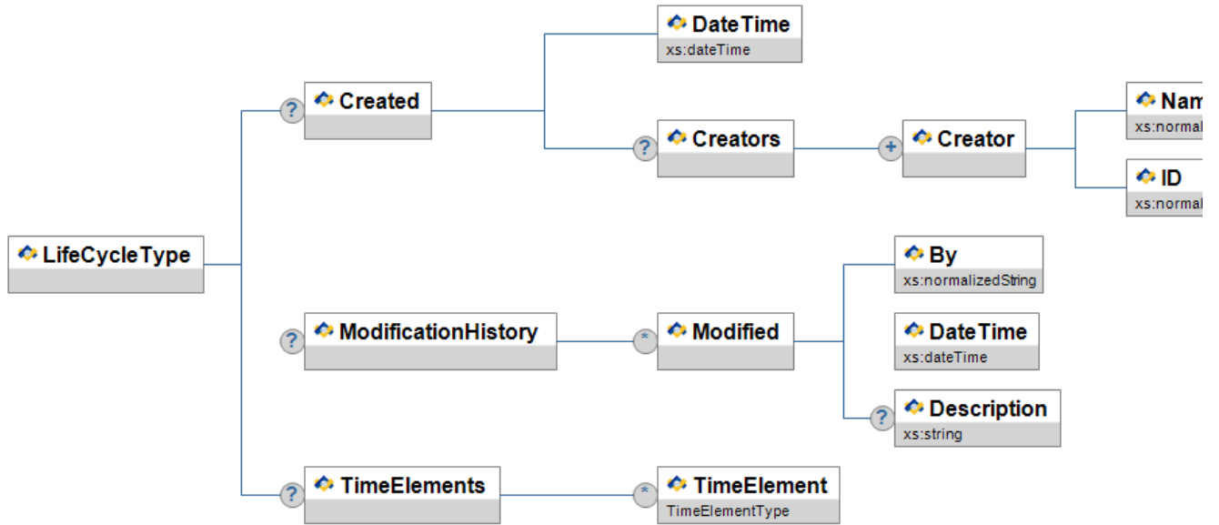
Figure A.107-1: LifeCycleType
