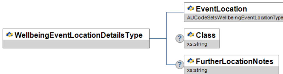
Figure A.276-1: WellbeingEventLocationDetailsType
