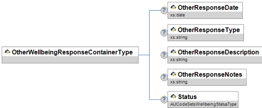
Figure A.150-1: OtherWellbeingResponseContainerType
