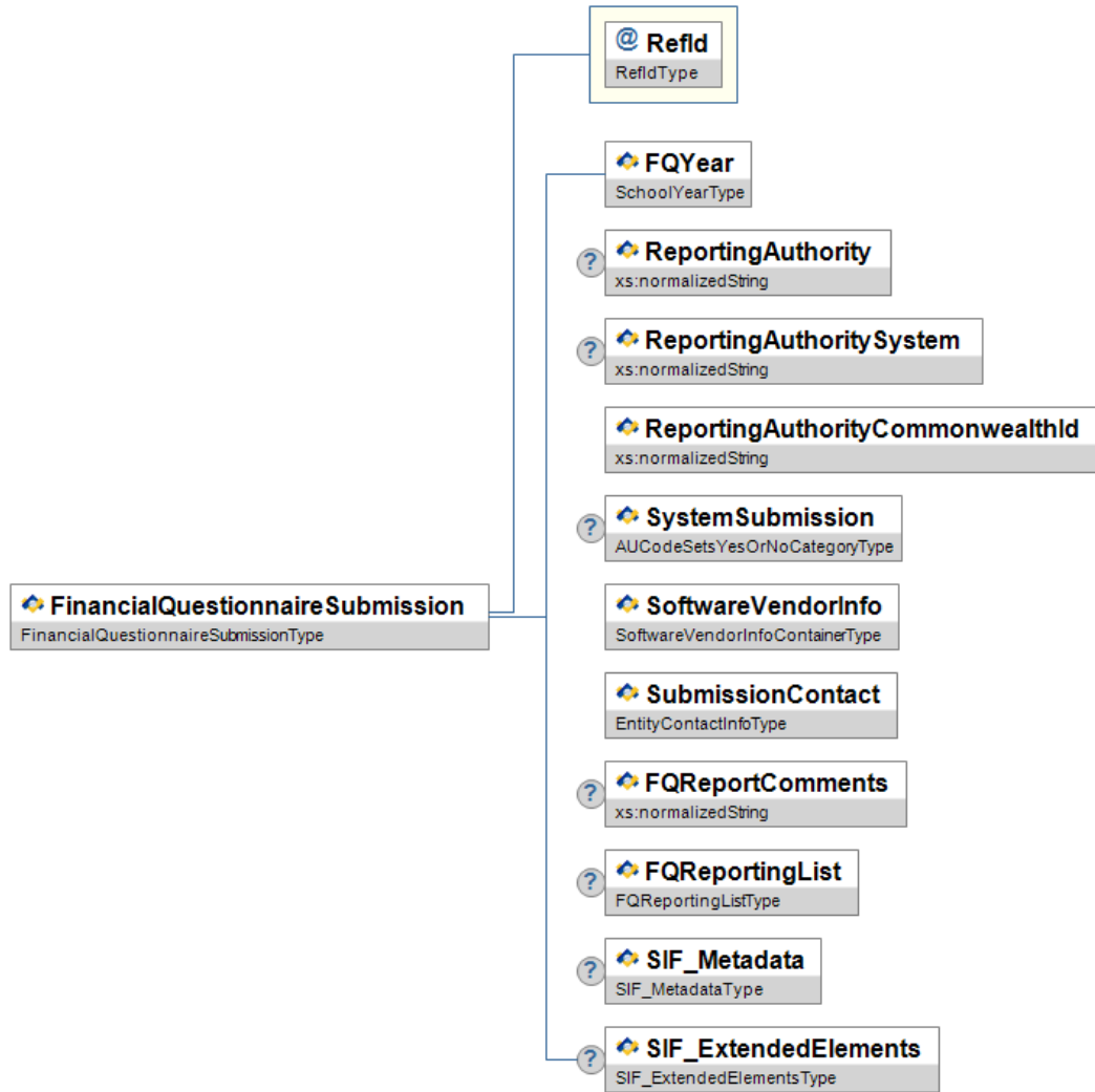
Figure 3.5.2-1: FinancialQuestionnaireSubmission
