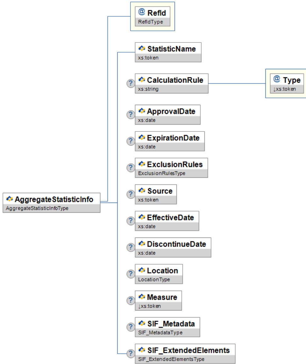
Figure 3.3.3-1: AggregateStatisticInfo
