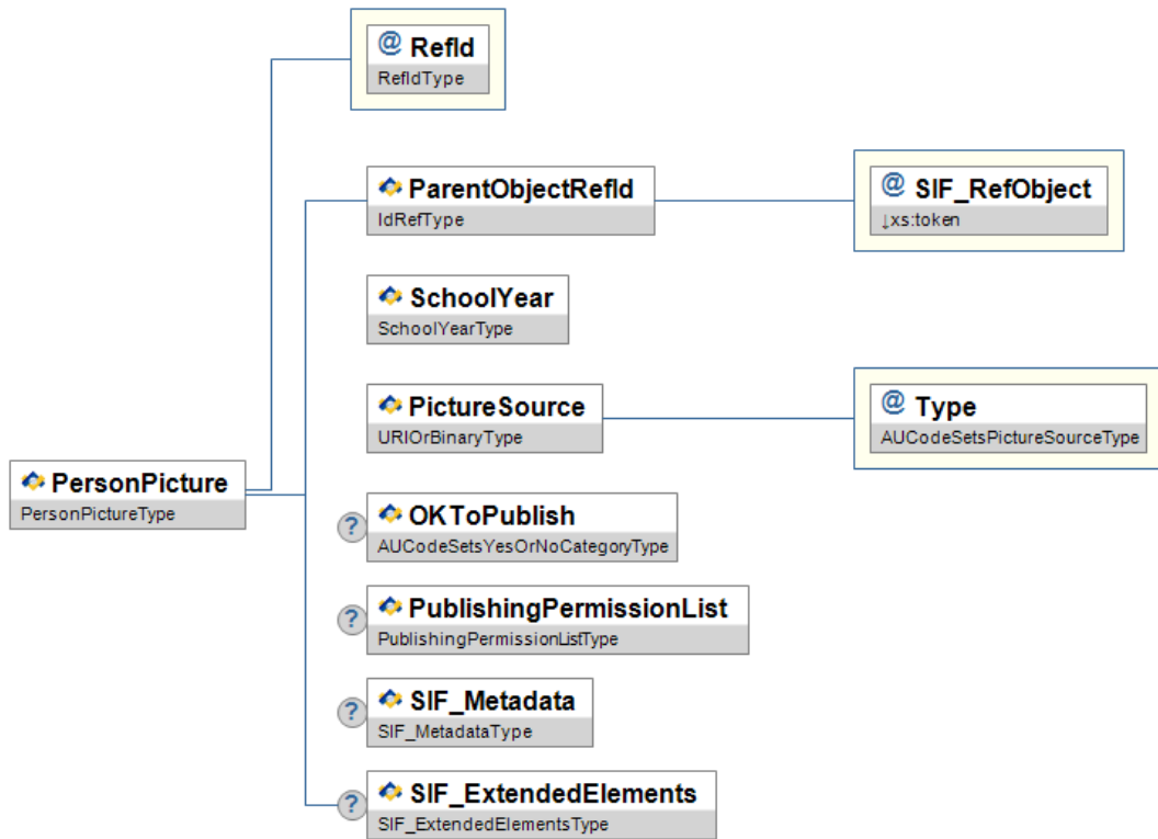
Figure 3.10.3-1: PersonPicture
