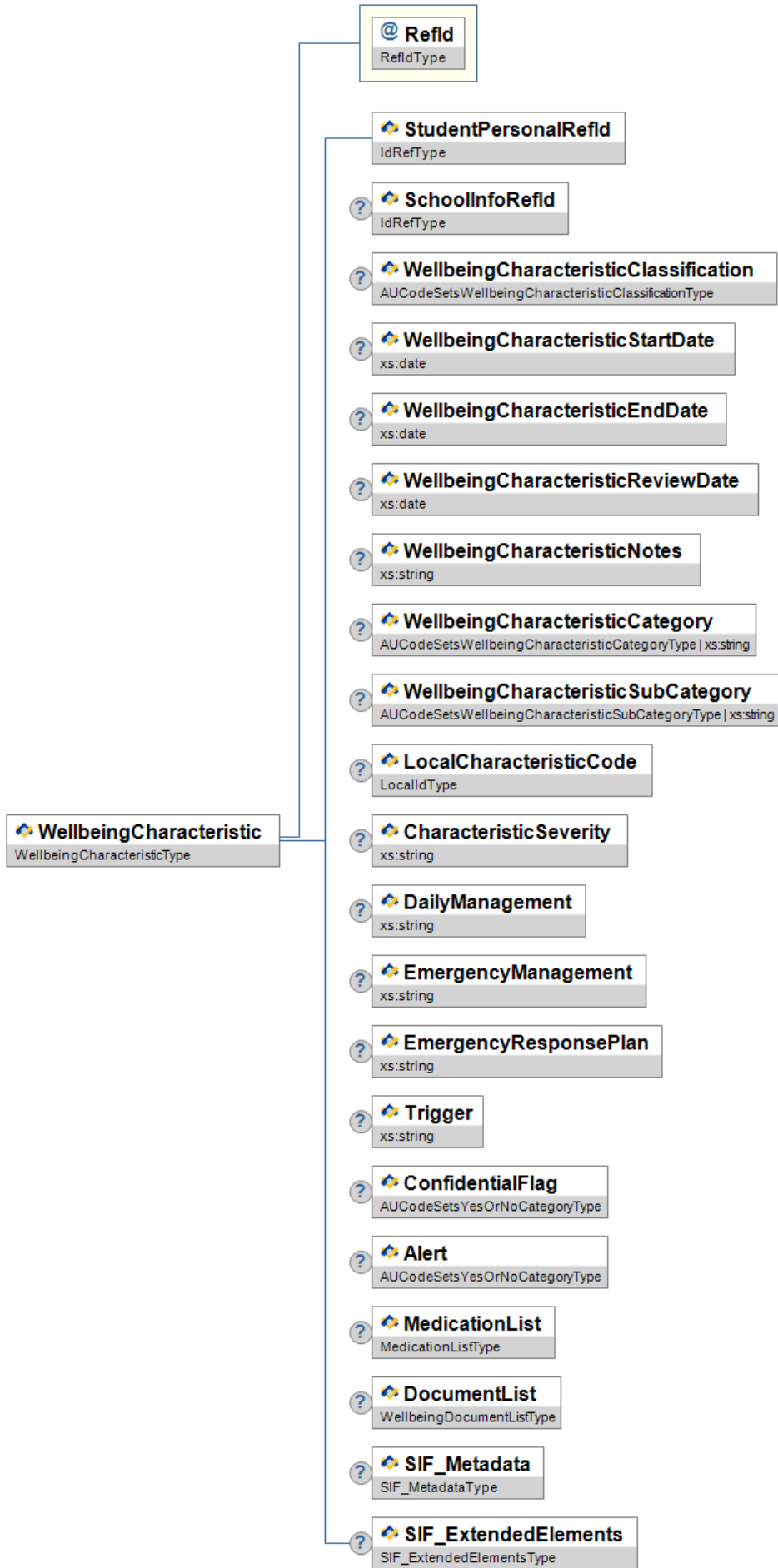
Figure 3.12.4-1: WellbeingCharacteristic
