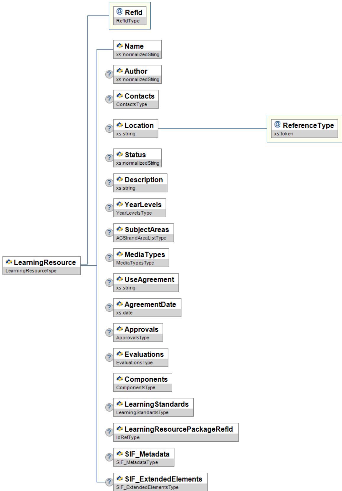
Figure 3.8.1-1: LearningResource
