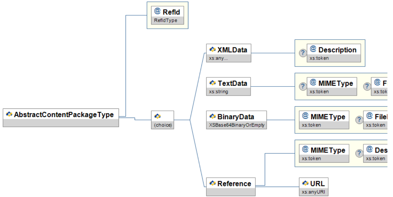
Figure A.2-1: AbstractContentPackageType
