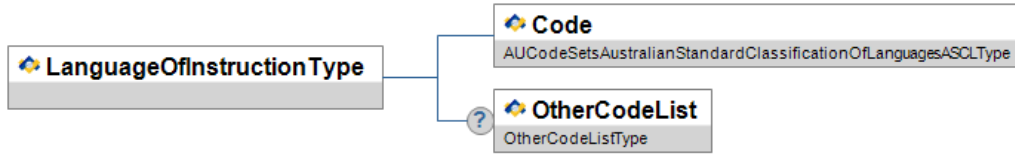
Figure A.98-1: LanguageOfInstructionType
