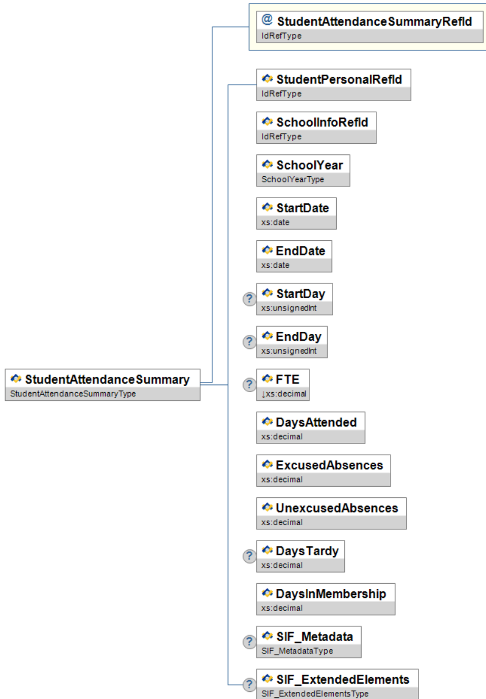
Figure 3.4.4-1: StudentAttendanceSummary
