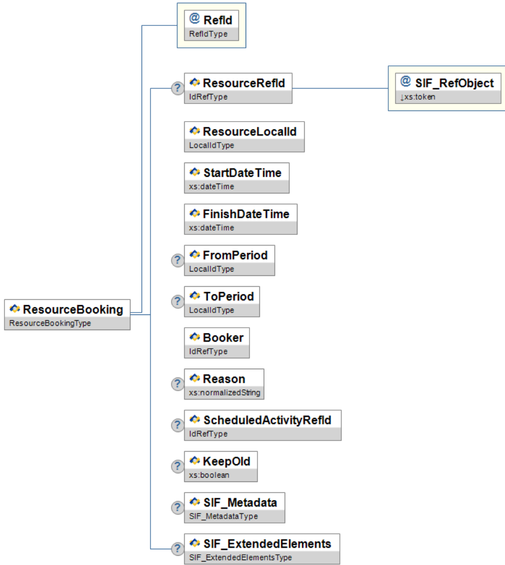
Figure 3.11.2-1: ResourceBooking
