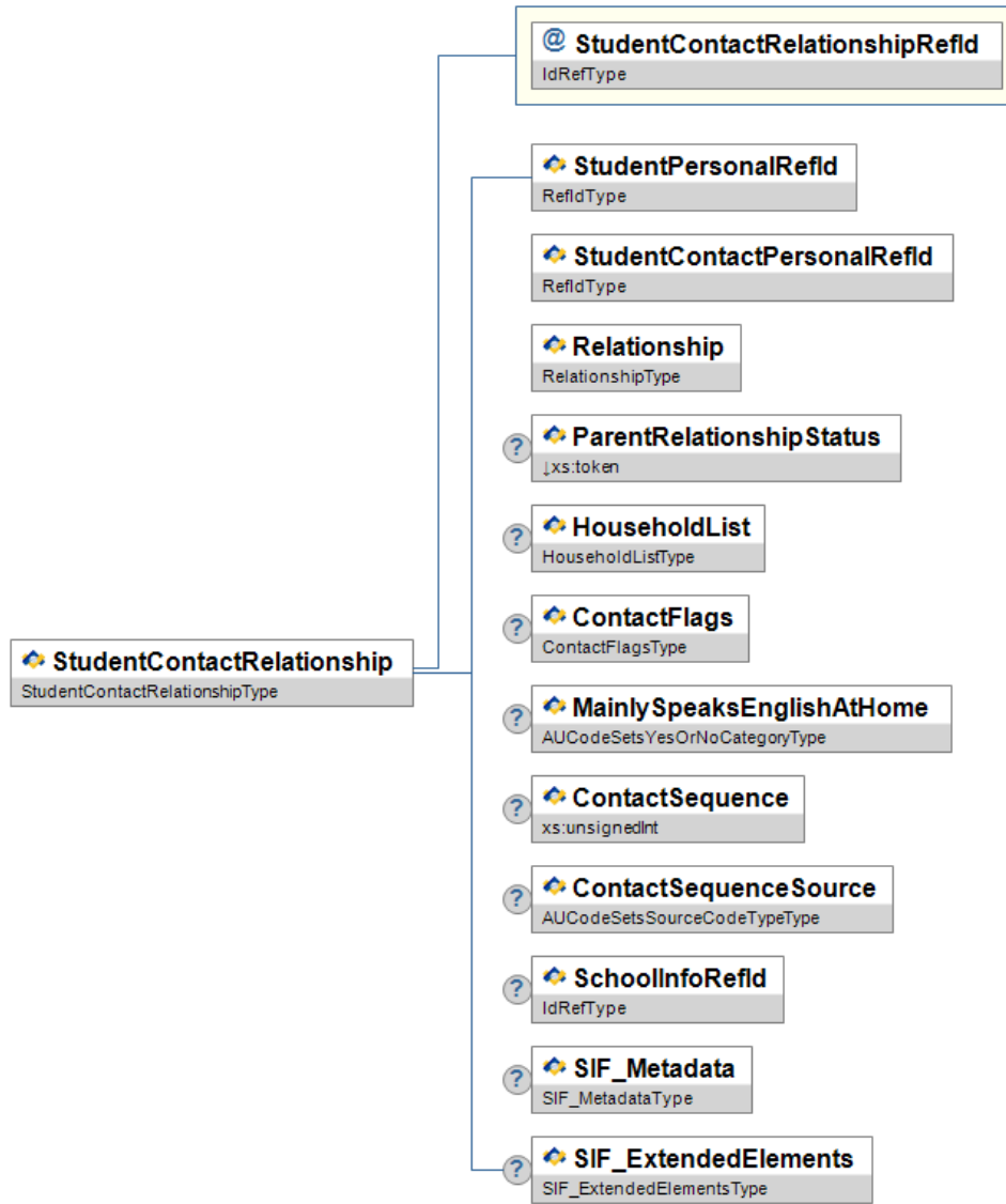
Figure 3.10.8-1: StudentContactRelationship
