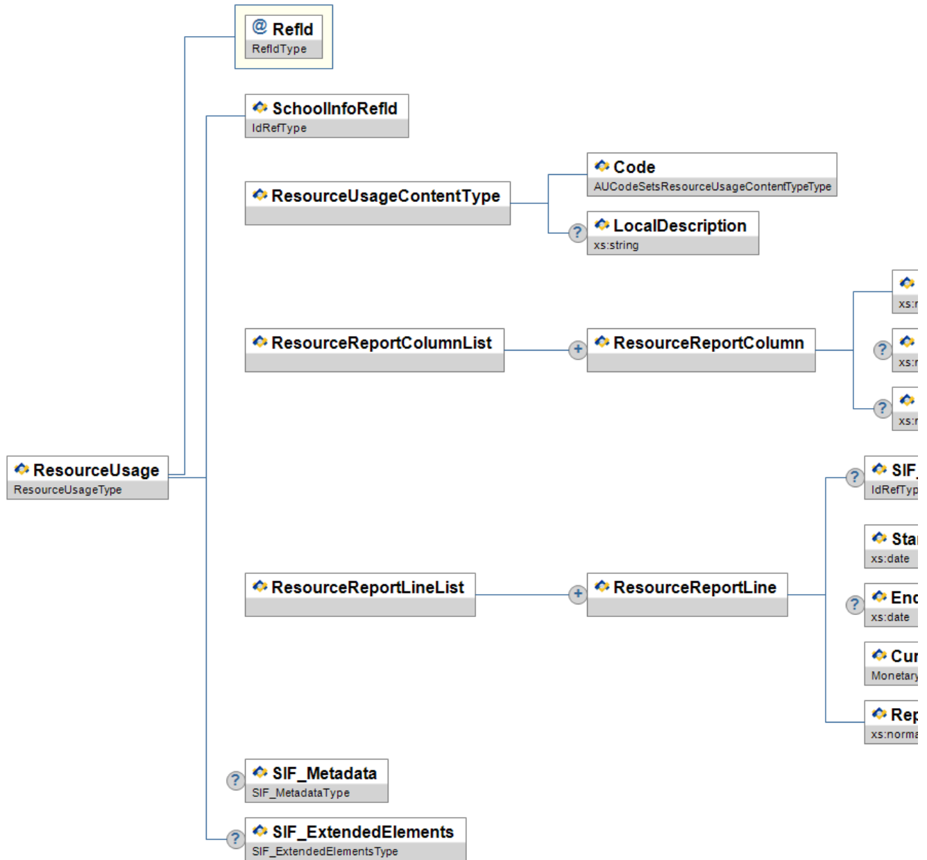
Figure 3.13.1-1: ResourceUsage
