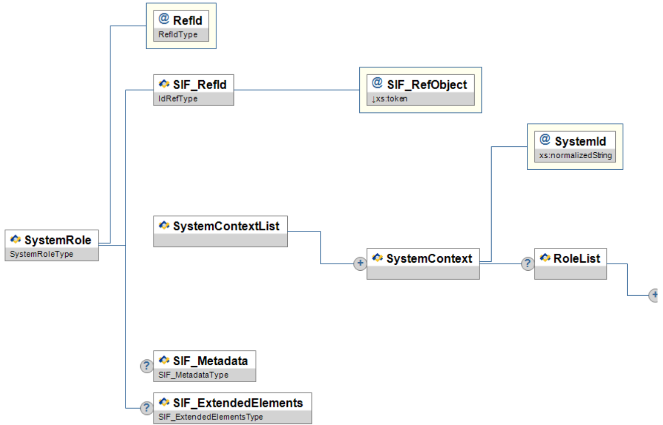
Figure 3.13.2-1: SystemRole
