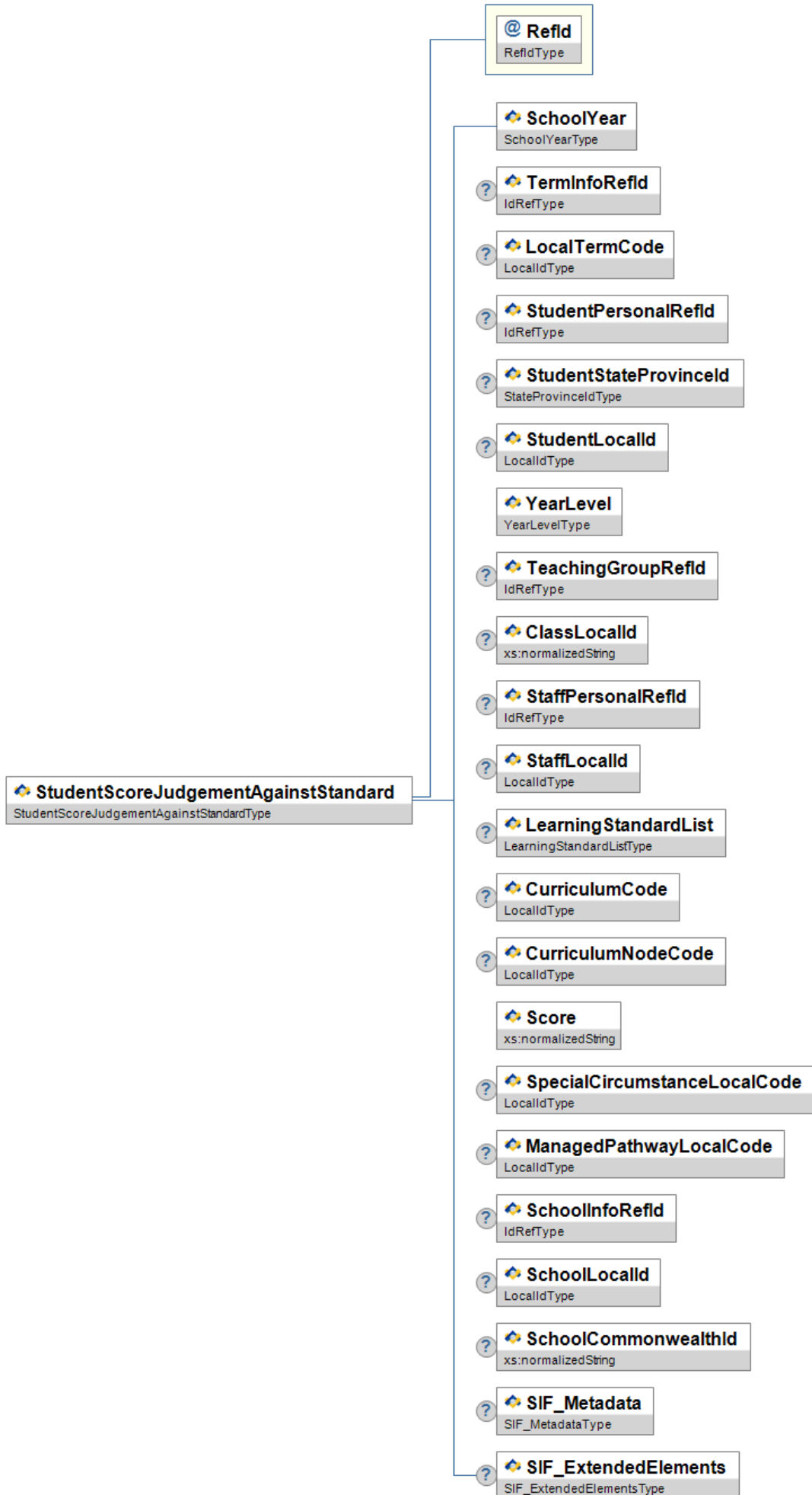
Figure 3.6.5-1: StudentScoreJudgementAgainstStandard
