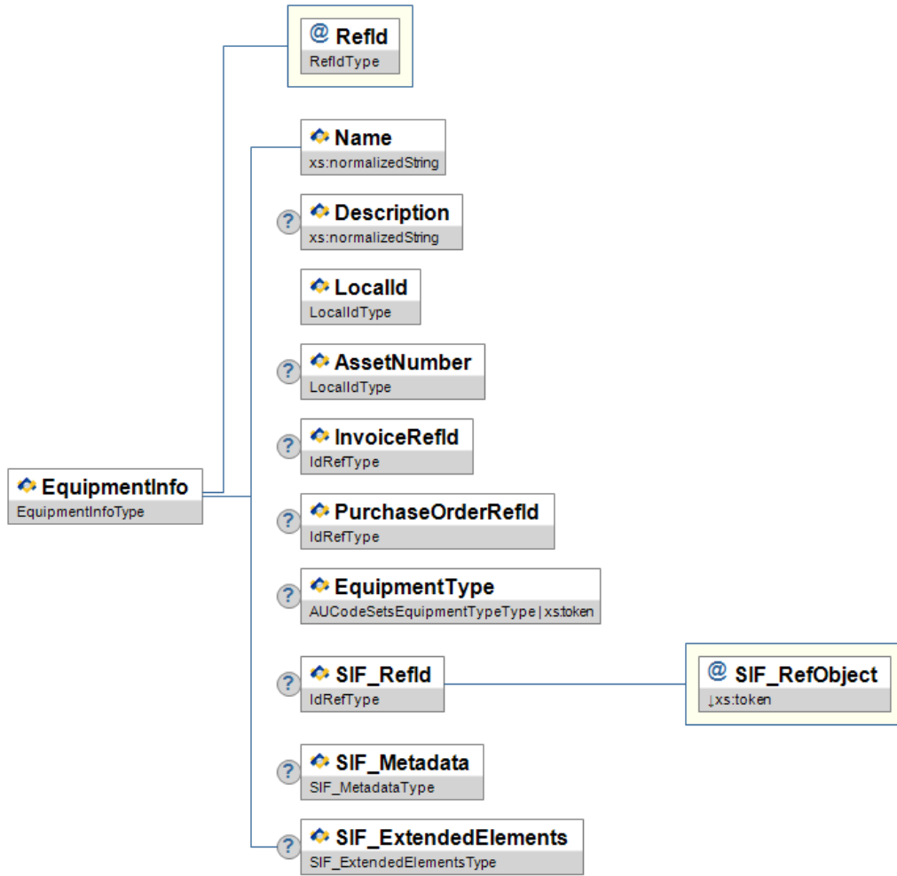
Figure 3.11.1-1: EquipmentInfo
