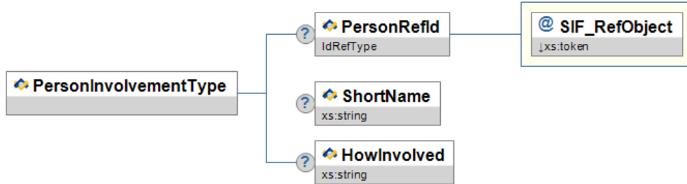
Figure A.157-1: PersonInvolvementType
