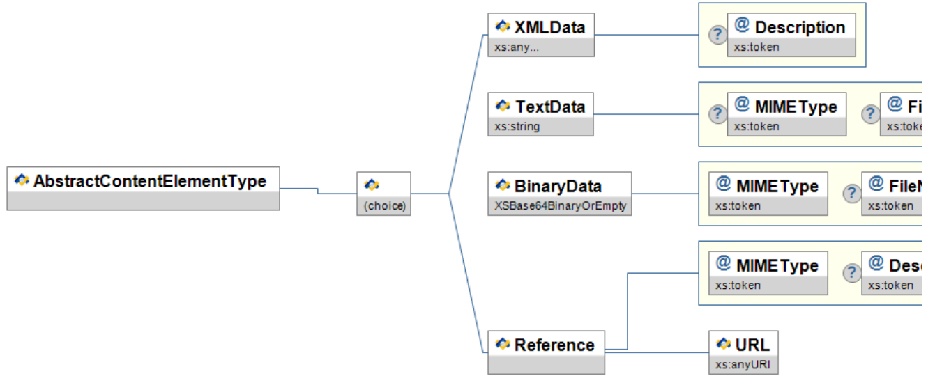
Figure A.1-1: AbstractContentElementType
